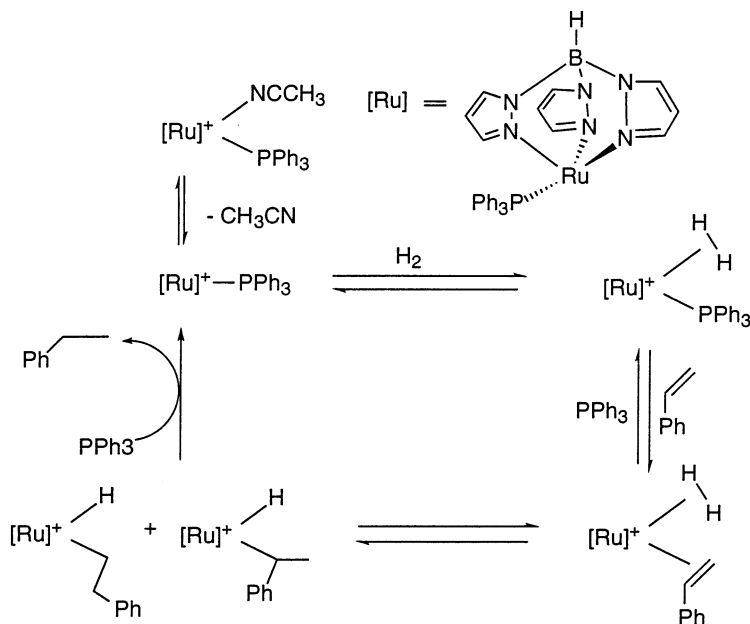
Scheme 6.
