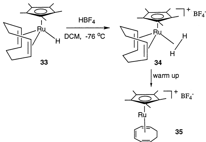
Scheme 7.
