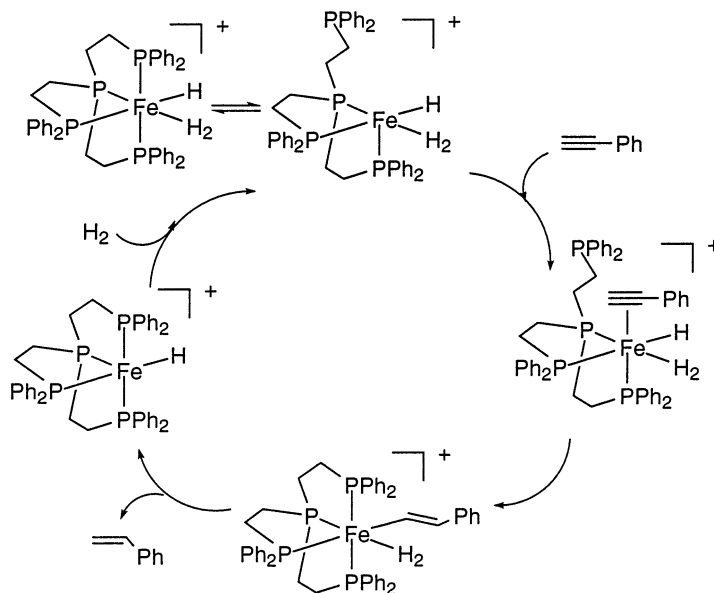
Scheme 5.
