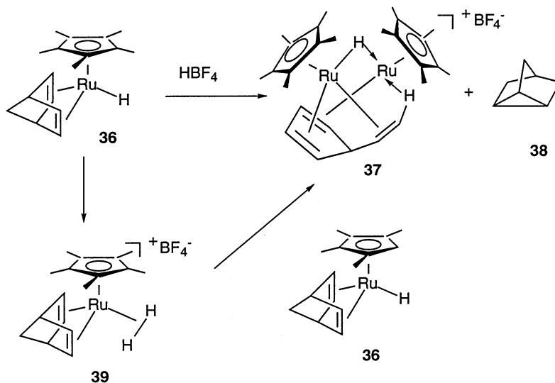
Scheme 8.
